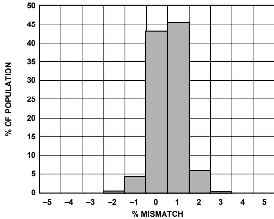
Figure 10. Self-Test Mismatch at 25°C ( V_{RATIO} = 5 V )
