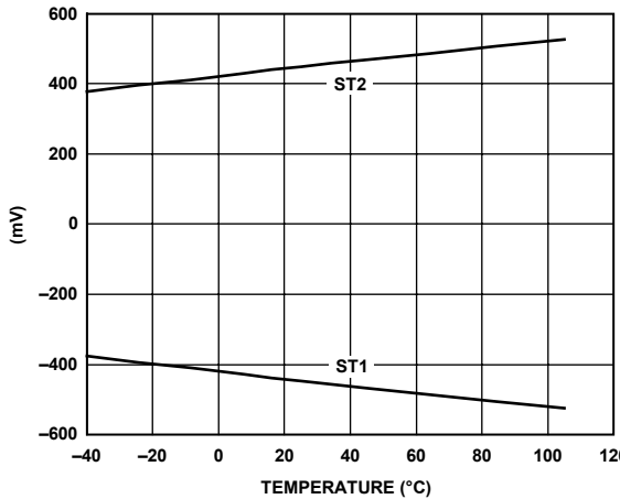
Figure 11. Typical Self-Test Change over Temperature
