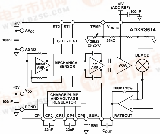
Figure 1. ADXRS614 Block Diagram
