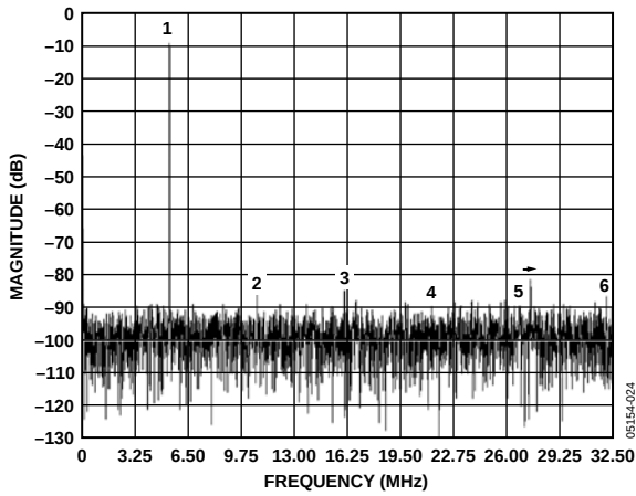
Figure 15. Single-Tone FFT of Channel B Digitizing f_{IN} = 70 MHz @ -9 dBFS While Channel A Digitizes f_{IN} = 70 MHz @ -9 dBFS
