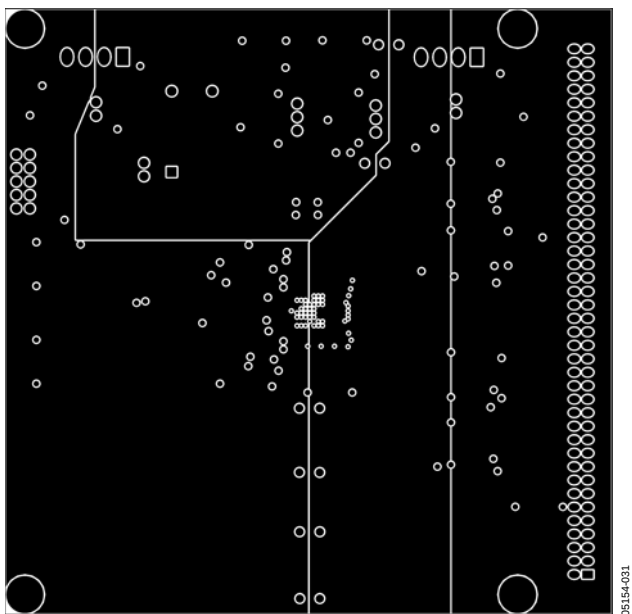
Figure 25. AD15252 Evaluation Board Power Plane
