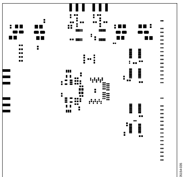
Figure 29. AD15252 Evaluation Board Bottom Paste
