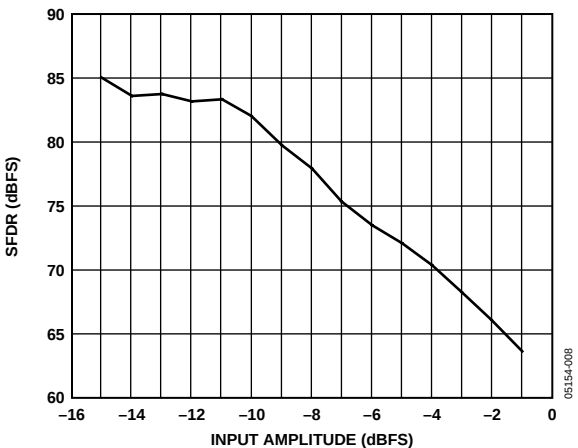
Figure 7. Single-Tone SFDR vs. AIN with f_{IN} = 110 MHz
