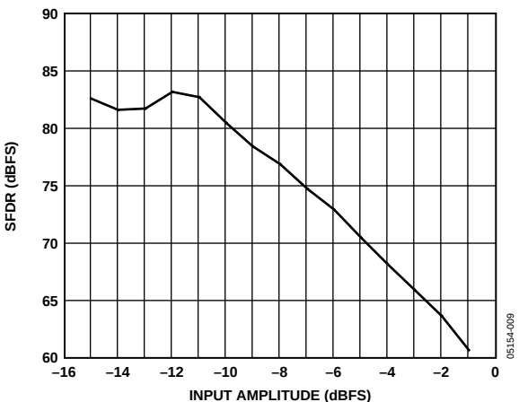
Figure 8. Single-Tone SFDR vs. AIN with f_{IN} = 140 MHz
