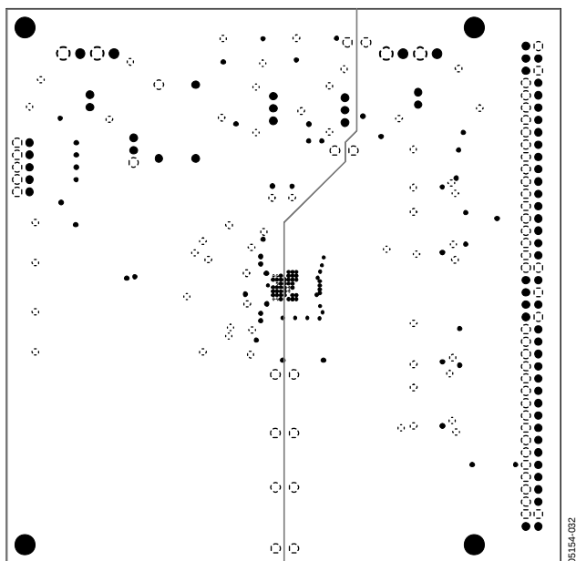
Figure 26. AD15252 Evaluation Board Ground Plane
