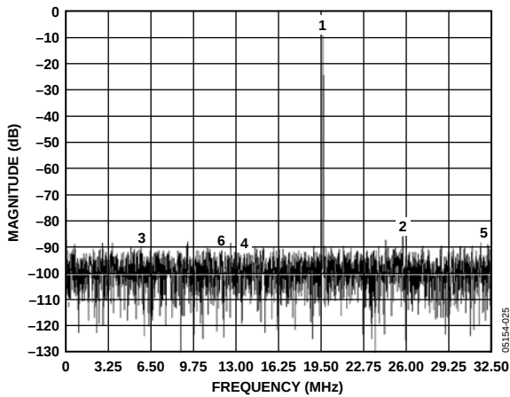
Figure 16. Single-Tone FFT of Channel A Digitizing f_{IN} = 110 MHz @ -9 dBFS While Channel B Digitizes f_{IN} = 110 MHz @ -9 dBFS
