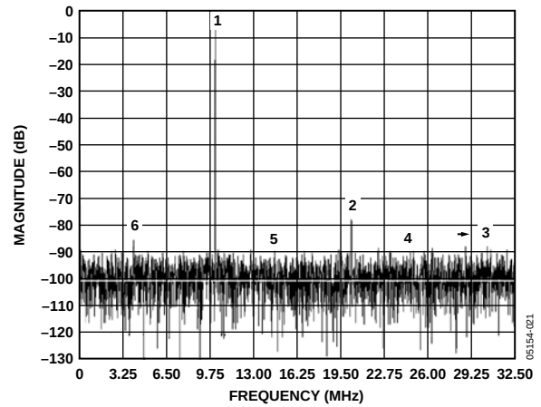
Figure 18. Single-Tone FFT of Channel A Digitizing f_{IN} = 140 MHz @ -9 dBFS While Channel B Digitizes f_{IN} = 140 MHz @ -9 dBFS
