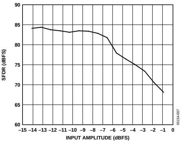
Figure 6. Single-Tone SFDR vs. AIN with f_{IN} = 70 MHz
