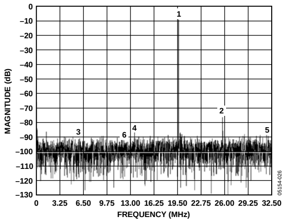
Figure 17. Single-Tone FFT of Channel B Digitizing f_{IN} = 110 MHz @ -9 dBFS While Channel A Digitizes f_{IN} = 110 MHz @ -9 dBFS
