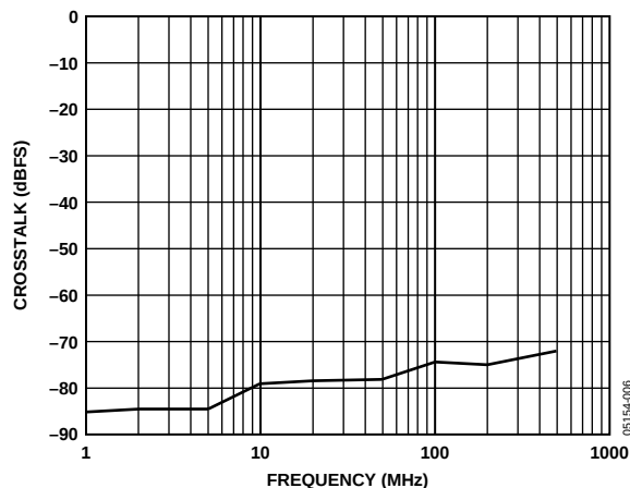
Figure 5. Typical Crosstalk
