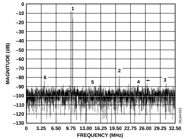
Figure 19. Single-Tone FFT of Channel B Digitizing f_{IN} = 140 MHz @ -9 dBFS While Channel A Digitizes f_{IN} = 140 MHz @ -9 dBFS
