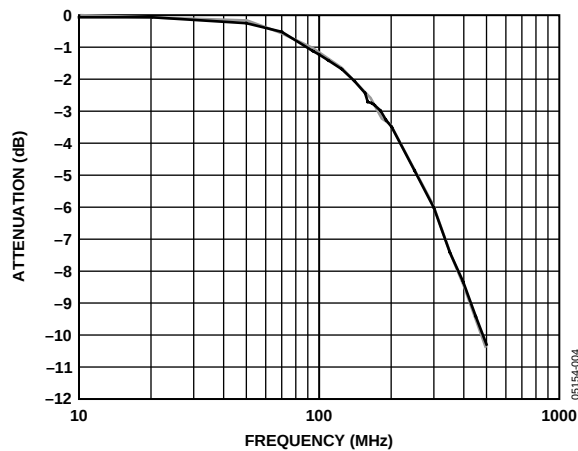
Figure 3. Gain Flatness
