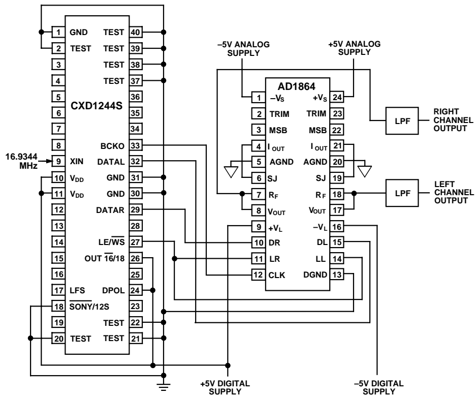
Figure 15. AD1864 with Sony CXD1244S Digital Filter
