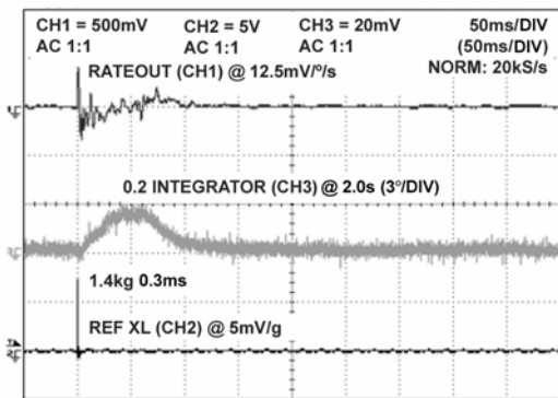
Figure 18. Hi-g Shock in Rate Axis (40 Hz)
