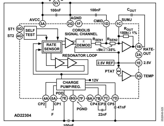
Figure 23. Block Diagram with External Components
