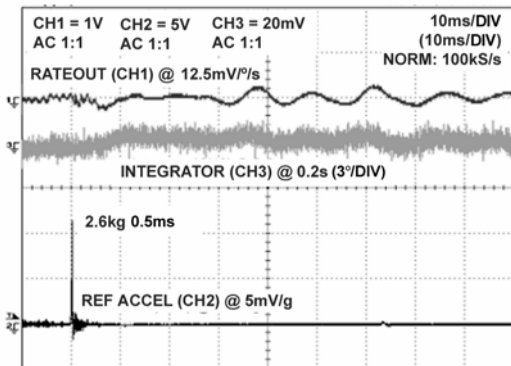
Figure 17. Hi-g Shock Test in Lateral Axis (40 Hz)
