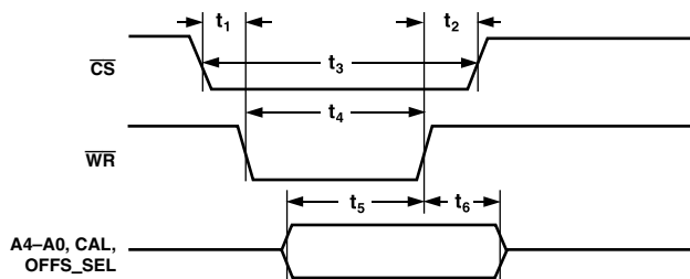
Figure 1. Parallel Write (ISHA Mode Only)
