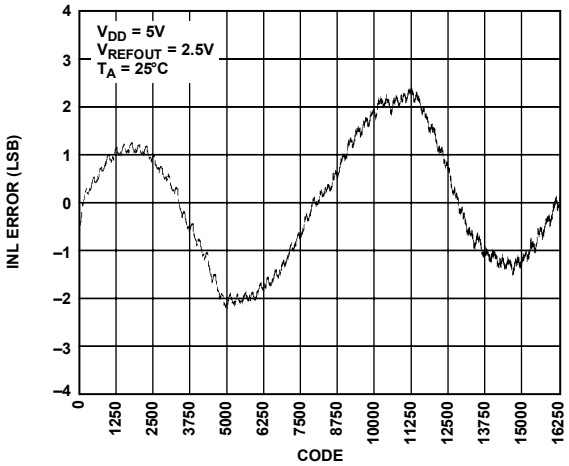
Figure 11. INL—AD5643R-5
