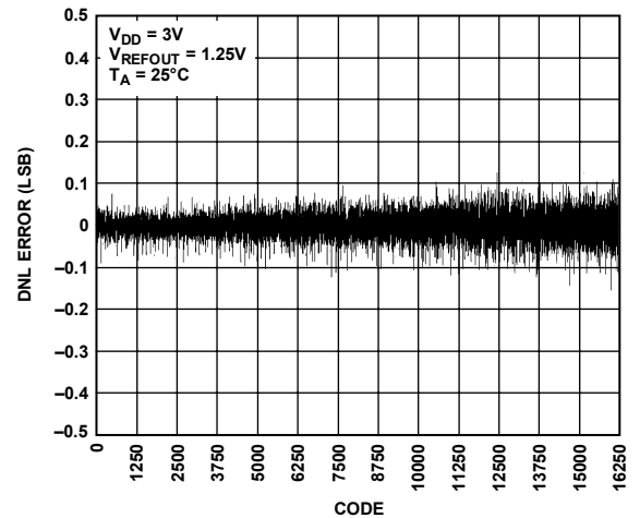
Figure 20. DNL—AD5643R-3
