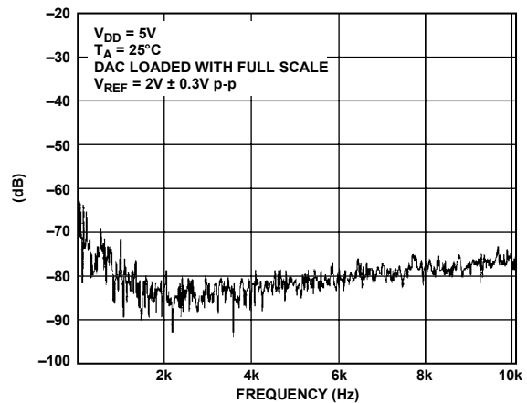
Figure 45. Total Harmonic Distortion
