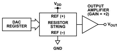
Figure 49. DAC Architecture
