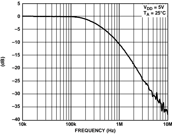
Figure 47. Multiplying Bandwidth
