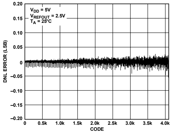
Figure 15. DNL—AD5623R-5
