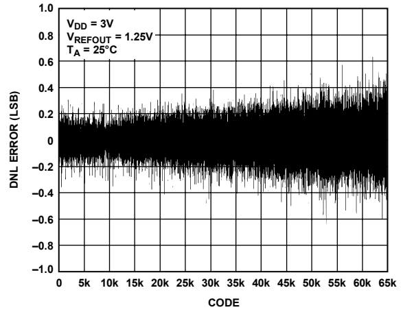
Figure 19. DNL—AD5663R-3
