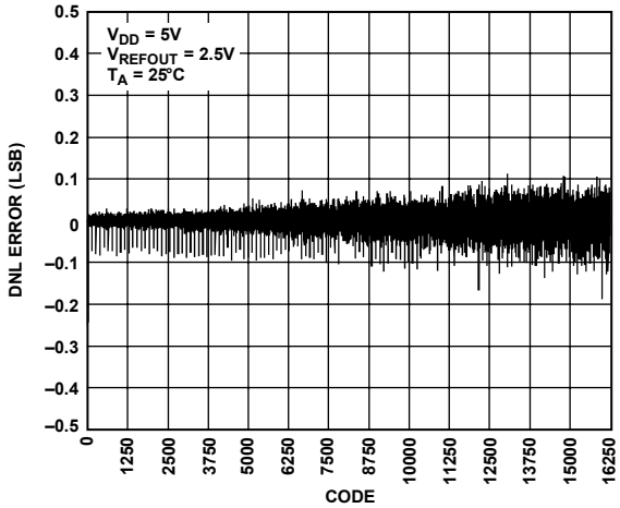
Figure 14. DNL—AD5643R-5
