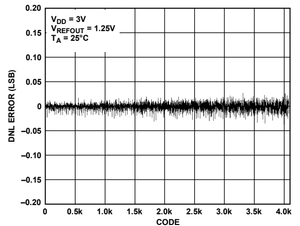
Figure 21. DNL—AD5623R-3
