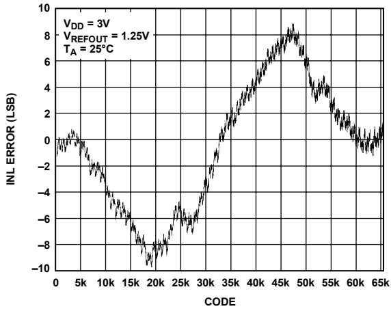
Figure 16. INL—AD5663R-3
