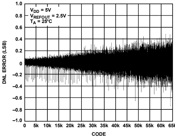
Figure 13. DNL—AD5663R-5
