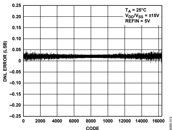
Figure 9. Differential Nonlinearity Error vs. Code, V_{DD}/V_{SS} = \pm 15\text{ V}
