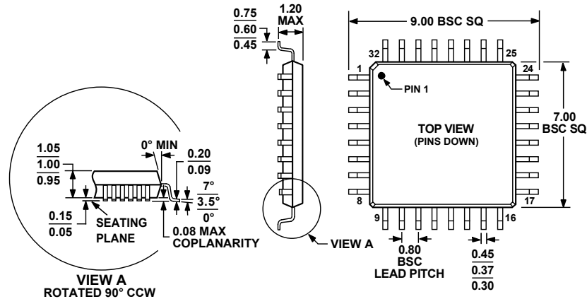
Figure 45. 32-Lead Thin Plastic Quad Flat Package [TQFP] (SU-32-2)
