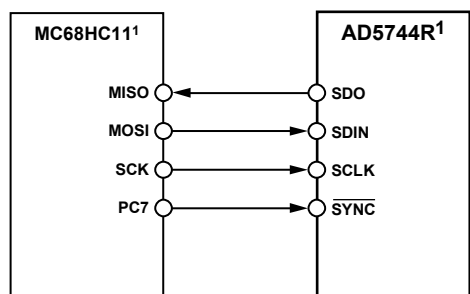
Figure 41. AD5744R to MC68HC11 Interface
