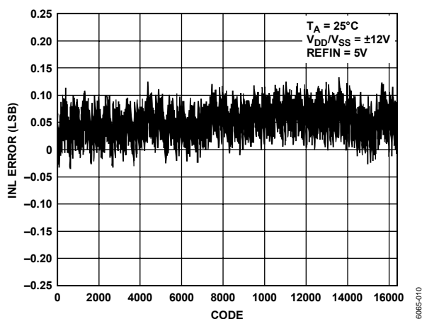
Figure 8. Integral Nonlinearity Error vs. Code, V_{DD}/V_{SS} = \pm 12\text{ V}
