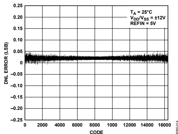
Figure 10. Differential Nonlinearity Error vs. Code, V_{DD}/V_{SS} = \pm 12\text{ V}
