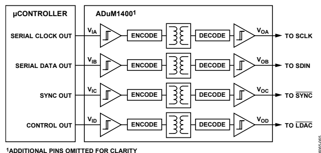
Figure 40. Isolated Interface
