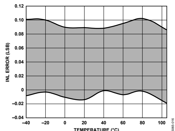
Figure 12. Integral Nonlinearity Error vs. Temperature, V_{DD}/V_{SS} = \pm 12\text{ V}
