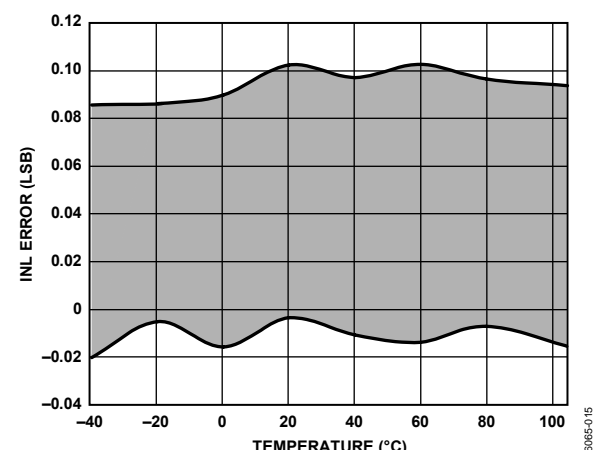
Figure 11. Integral Nonlinearity Error vs. Temperature, V_{DD}/V_{SS} = \pm 15\text{ V}
