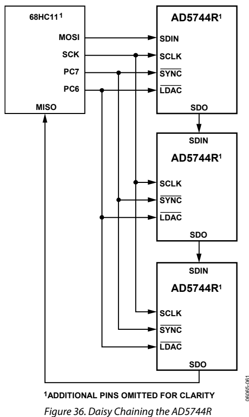
Figure 36. Daisy Chaining the AD5744R
