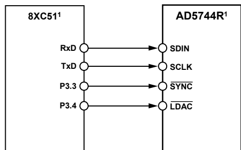
Figure 42. AD5744R to 8XC51 Interface
