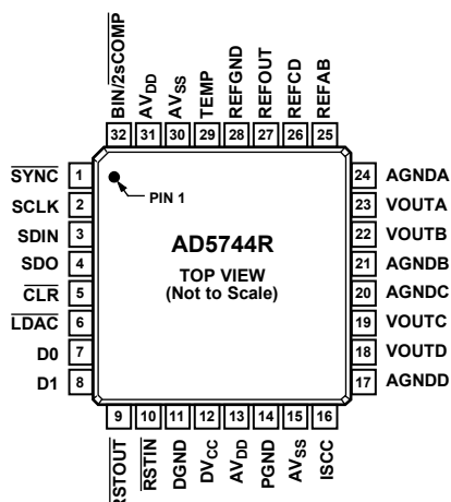
Figure 6. Pin Configuration
