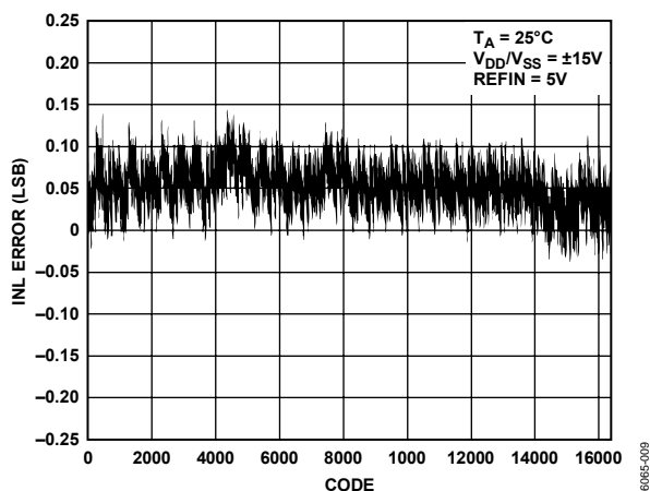
Figure 7. Integral Nonlinearity Error vs. Code, V_{DD}/V_{SS} = \pm 15\text{ V}
