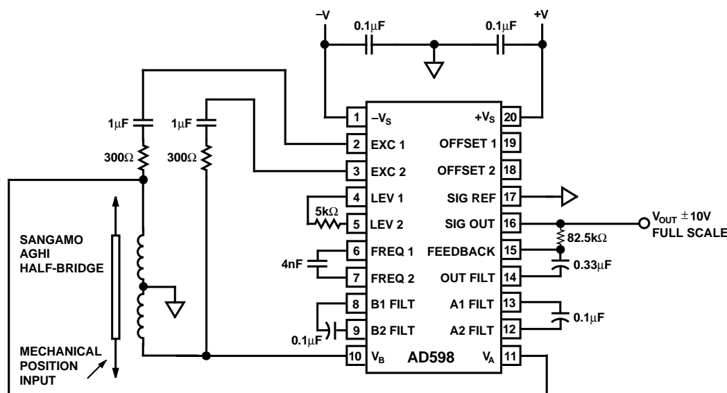
Figure 27. Half-Bridge Operation
