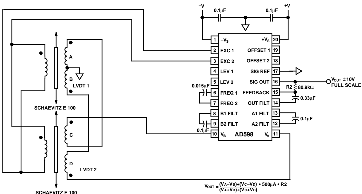
Figure 25. Differential Gaging
