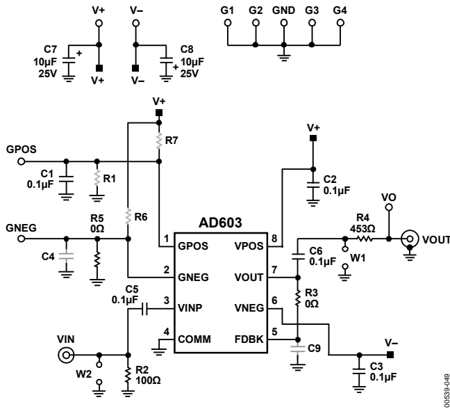
Figure 49. Schematic of the AD603 Evaluation Board
