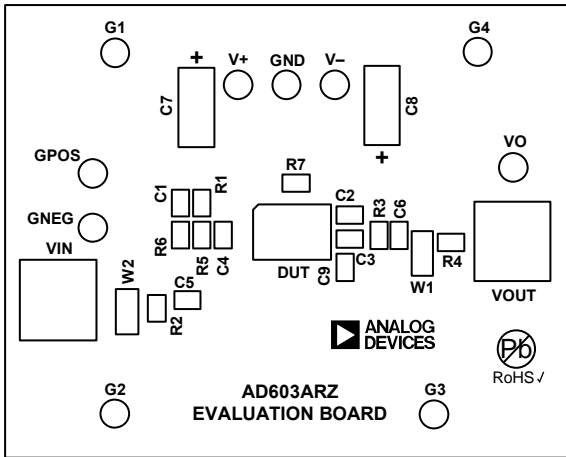
Figure 52. Component Side Silk Screen
