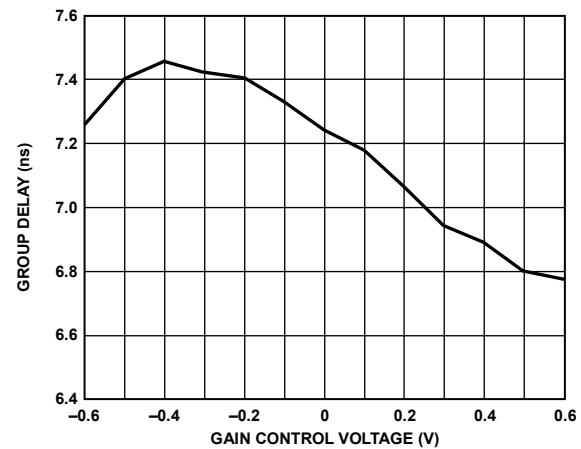
Figure 9. Group Delay vs. Gain Control Voltage
