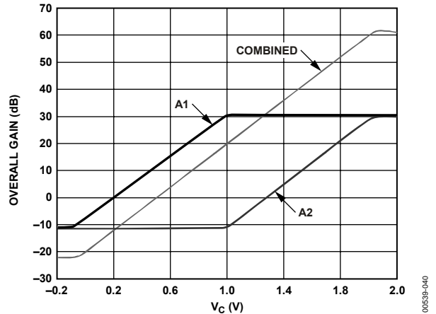
Figure 40. Plot of Separate and Overall Gains in Sequential Control
