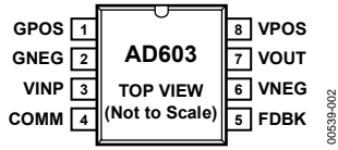
Figure 2. 8-Lead SOIC Pin Configuration
