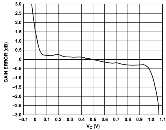
Figure 45. Gain Error for Cascaded Stages—Low Ripple Mode
