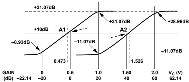
Figure 39. Explanation of Offset Calibration for Sequential Control
