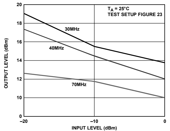
Figure 27. Third-Order Intercept -10 dB/+30 dB Mode, Gain = 10 dB
