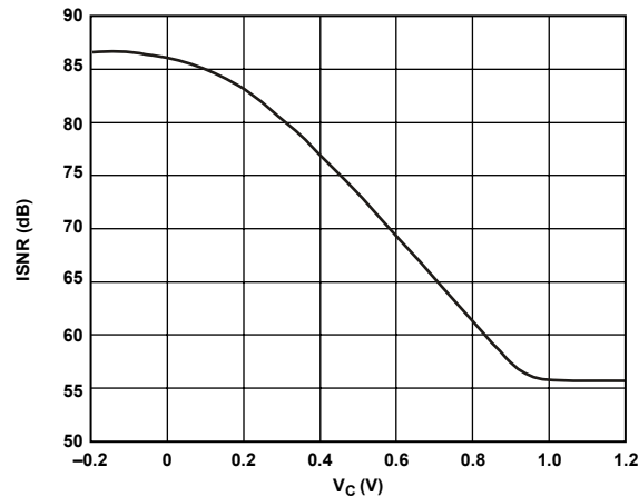
Figure 46. ISNR vs. Control Voltage—Low Ripple Mode
