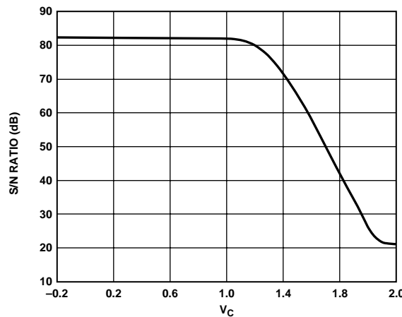
Figure 41. SNR for Cascaded Stages—Sequential Control
