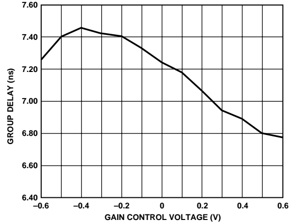
Figure 9. Group Delay vs. Gain Control Voltage
