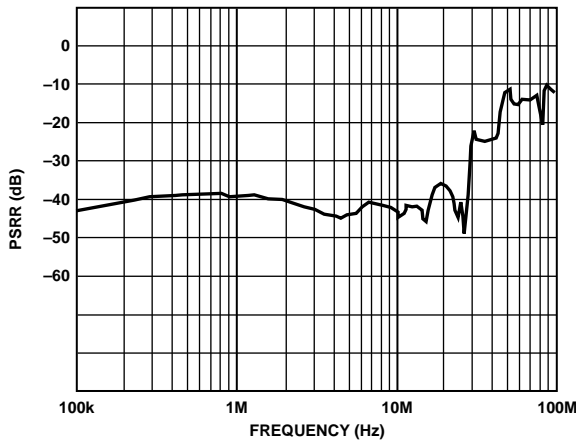
Figure 22. PSRR vs. Frequency (Worst Case is Negative Supply PSRR, Shown Here)
