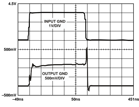
Figure 18. Input Stage Overload Recovery Time (Input is 500 ns Period, 50% Duty Cycle Square Wave, Output is Captured Using Tektronix 11402 Digitizing Oscilloscope)
