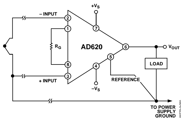
Figure 48. Ground Returns for Bias Currents with Thermocouple Inputs
