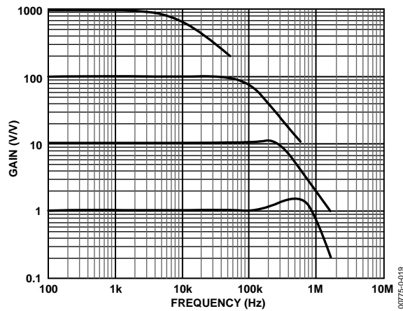
Figure 19. Gain vs. Frequency
