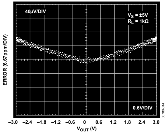
Figure 13. Gain Nonlinearity; V_S = \pm 5V , R_L = 1k\Omega
