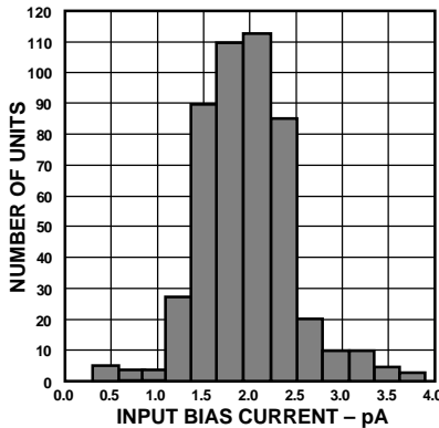
Figure 5. Typical Distribution of Input Bias Current (573 Units)
