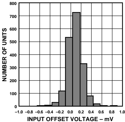
Figure 4. Typical Distribution of Input Offset Voltage (1255 Units)
