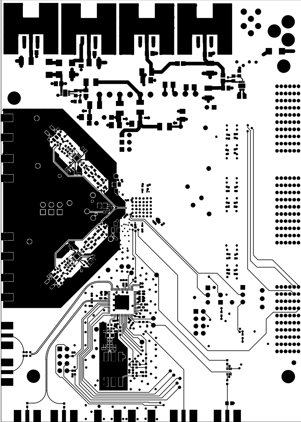
Figure 100. Evaluation Board Layout, Secondary Side (Mirrored Image)
