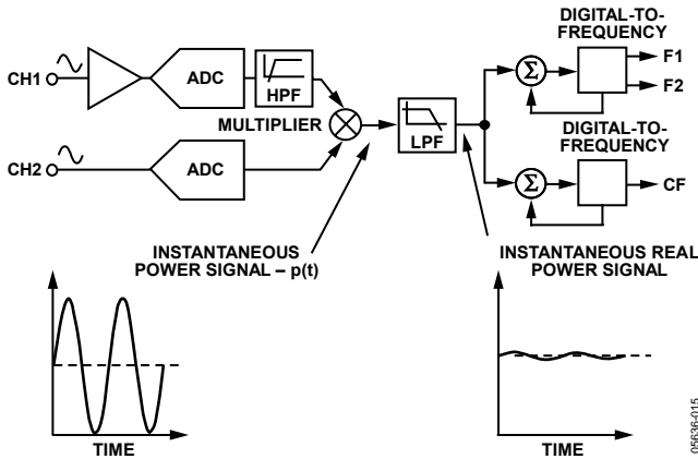
Figure 15. Signal Processing Block Diagram
