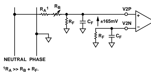
Figure 20. Typical Connections for Channel V2
