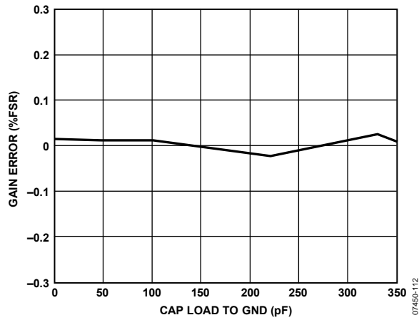
Figure 12. Capacitance Input Error vs. Capacitance Between EXC and GND, Differential Mode, C_{IN(+)} \text{ to EXC} = 8 \text{ pF} , C_{IN(-)} \text{ to EXC} = 6 \text{ pF} , V_{DD} = 3.3 \text{ V}
