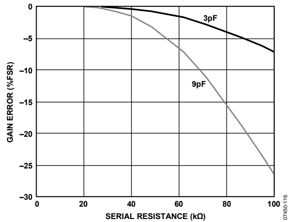
Figure 16. Capacitance Input Error vs. Serial Resistance, Single-Ended Mode, C_{IN(+)} \text{ to EXC} = 3 \text{ pF} and 9 \text{ pF} , V_{DD} = 3.3 \text{ V}
