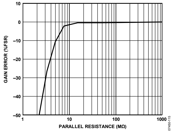
Figure 15. Capacitance Input Error vs. Parasitic Parallel Resistance Single-Ended Mode, C_{IN(+)} \text{ to EXC} = 9 \text{ pF} , V_{DD} = 3.3 \text{ V}
