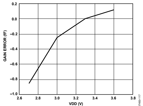
Figure 17. Capacitance Input Power Supply Rejection (PSR), Differential Mode; C_{IN(+)} \text{ to EXC} = 1.9 \text{ pF}
