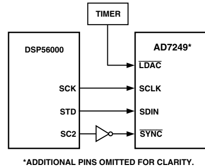
Figure 12. AD7249–DSP56000 Interface
