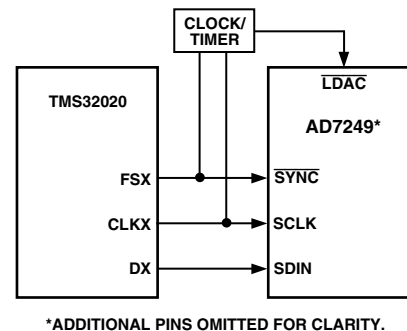
Figure 13. AD7249–TMS32020 Interface
