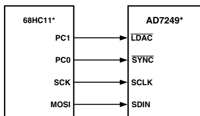
Figure 14. AD7249–68HC11 Interface
