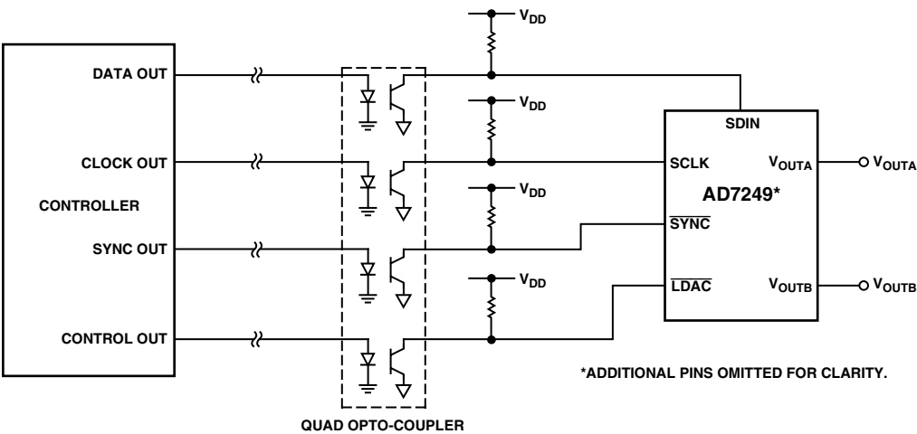
Figure 16. Opto-Isolated Interface
