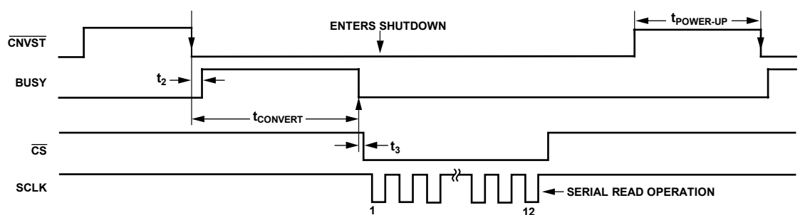
Figure 24. Autoshtutdown Mode for AD7366
