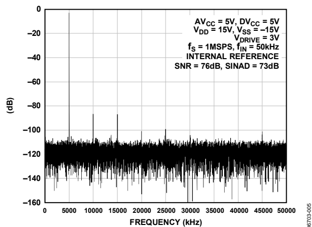
Figure 5. AD7367 FFT
