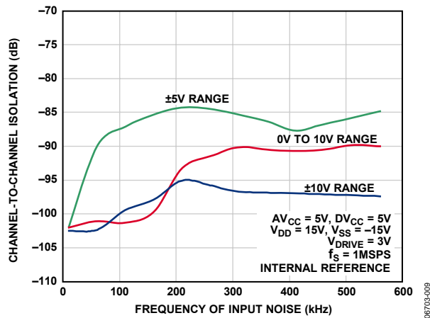
Figure 9. Channel-to-Channel Isolation
