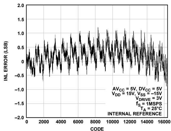
Figure 4. AD7367 Typical INL
