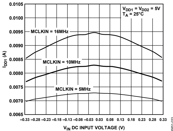
Figure 14. I_{DD1} vs. V_{IN}
