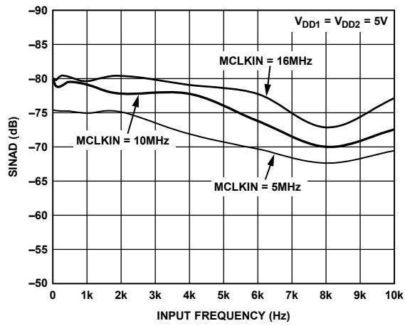
Figure 7. SINAD vs. Analog Input Frequency
