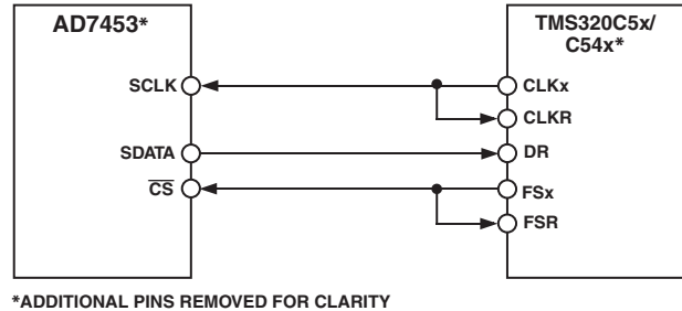
Figure 18. Interfacing to the TMS320C5x/C54x
