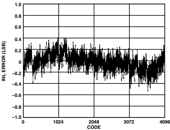
TPC 5. Typical INL For the AD7453 for V_{DD} = 5\text{ V}
