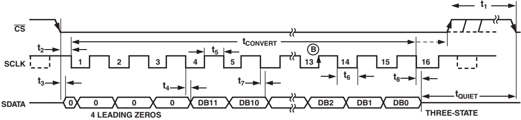
Figure 1. AD7453 Serial Interface Timing Diagram
