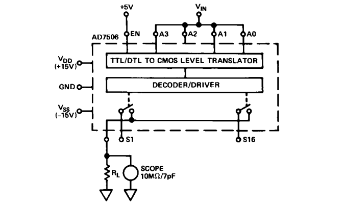
TEST CIRCUIT 1
