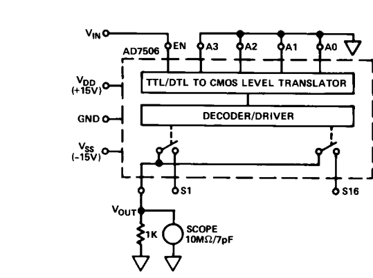
TEST CIRCUIT 2
