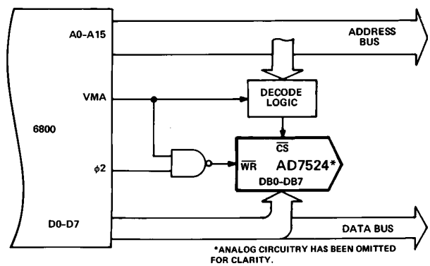
Figure 7. AD7524/MC6800 Interface
