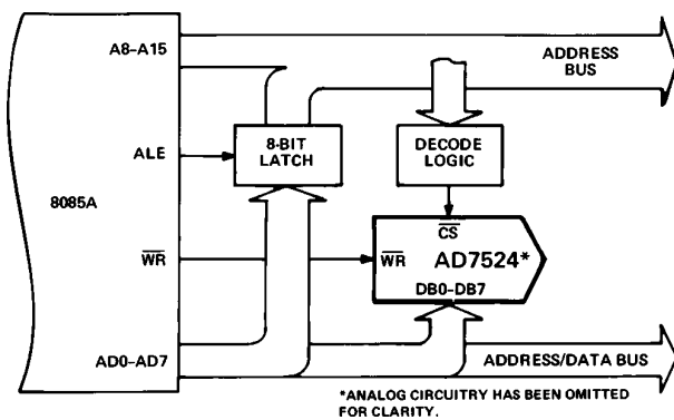
Figure 6. AD7524/8085A Interface
