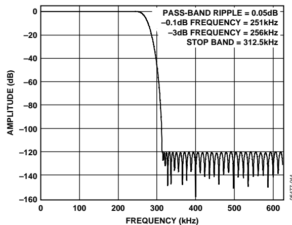
Figure 31. Default Filter Frequency Response (625 kHz ODR)
