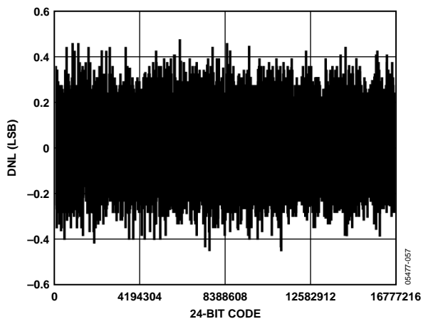
Figure 19. 24-Bit DNL
