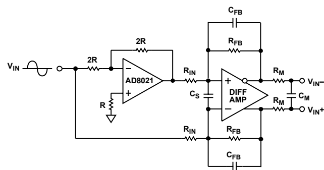
Figure 30. Single-Ended-to-Differential Conversion
