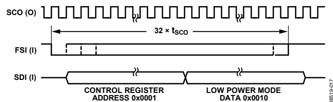
Figure 33. Write Scheme for Low Power Mode
