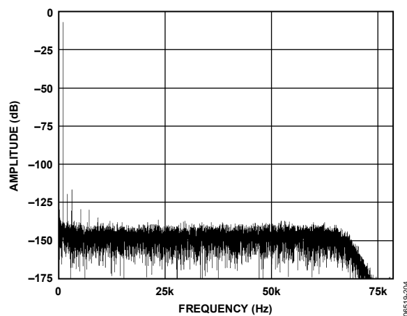
Figure 11. Low Power Mode; FFT, 1 kHz, - dB Input Tone, 128 \times Decimation Rate
