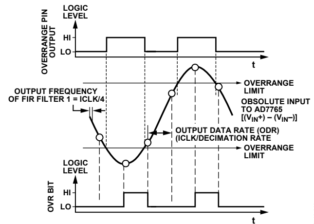
Figure 32. OVERRANGE Pin and OVR Bit vs. Absolute Voltage Applied to Modulator
