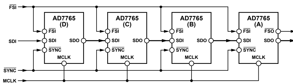
Figure 36. Writing to AD7765 Daisy-Chain Configuration
