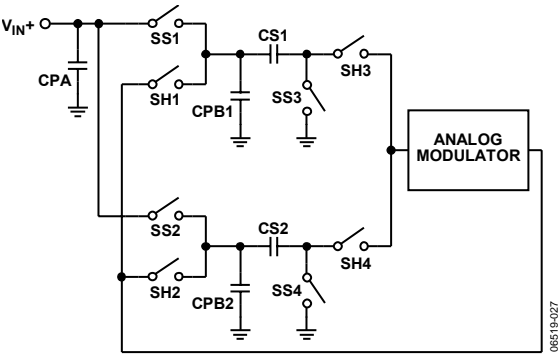
Figure 31. Equivalent Input Circuit
