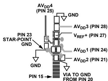
Figure 40. AD7765 Supply Decoupling
