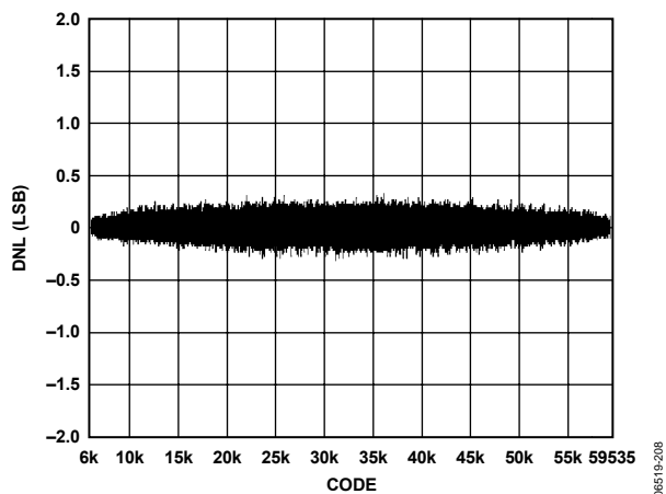
Figure 20. DNL Plot
