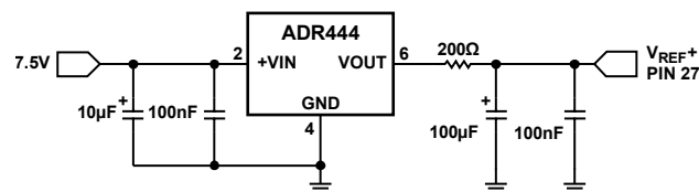
Figure 41. Reference Connection
