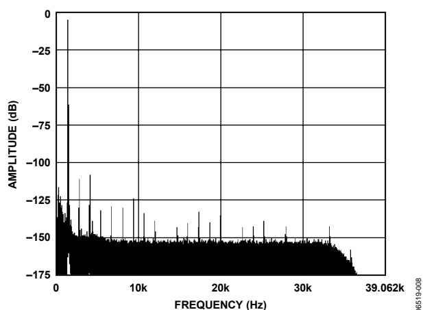
Figure 7. Normal Power Mode; FFT, 1 kHz, -0.5 dB Input Tone, 256 \times Decimation Rate
