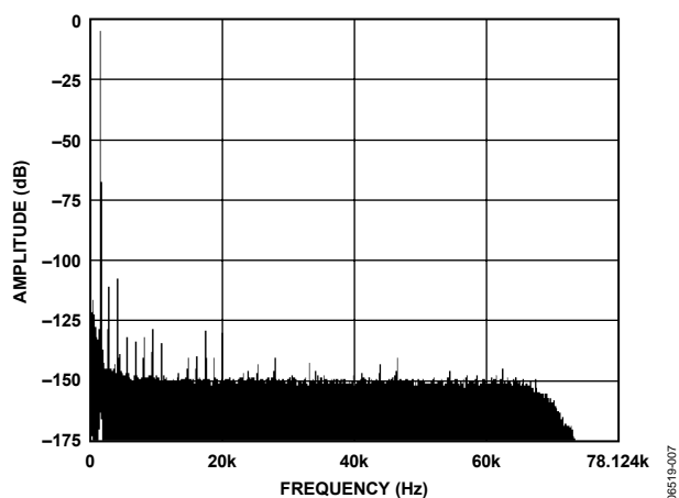
Figure 6. Normal Power Mode; FFT, 1 kHz, -0.5 dB Input Tone, 128 \times Decimation Rate
