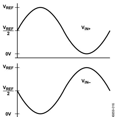
Figure 39. Maximum Differential Inputs to the AD7767
