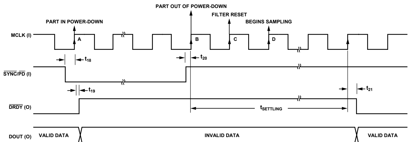
Figure 5. Reset, Synchronization, and Power-Down Timing Diagram
