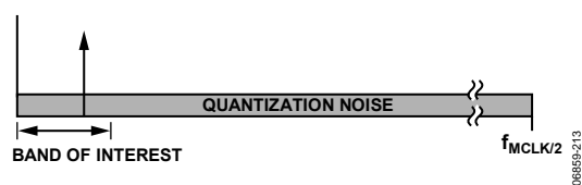
Figure 29. Quantization Noise
