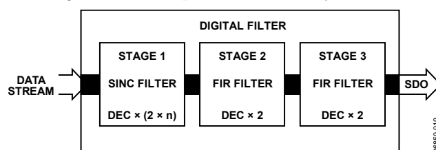
Figure 31. FIR Filter Stages ( n = 1 for AD7767, n = 2 for AD7767-1, n = 4 for AD7767-2)
