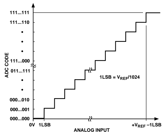
Figure 11. Transfer Characteristic
