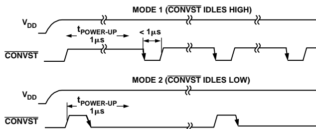
Figure 12. Power-Up Times
