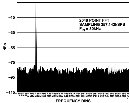
Figure 3. AD7810 SNR
