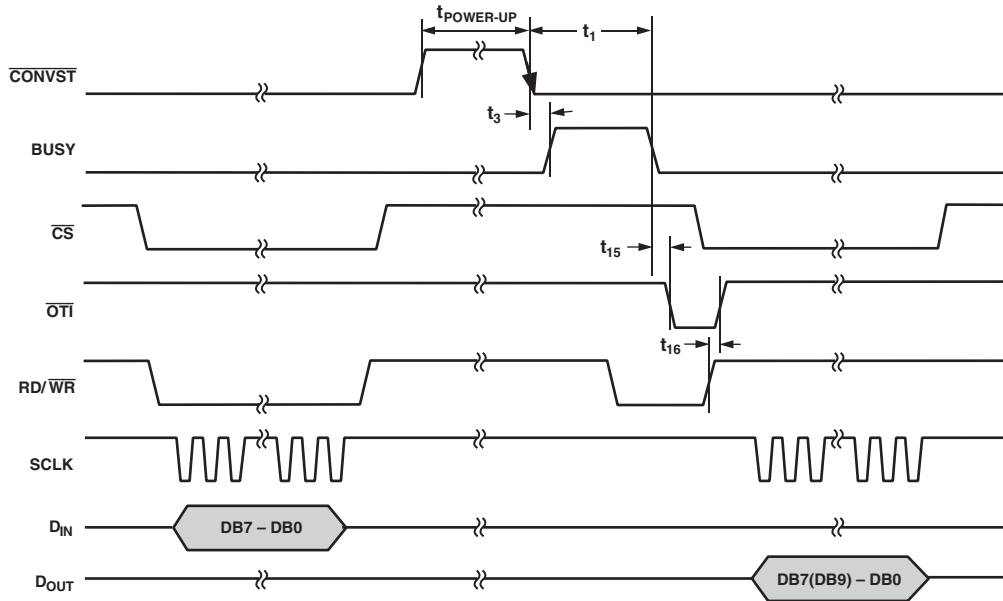
Figure 17. Mode 2 Operation
