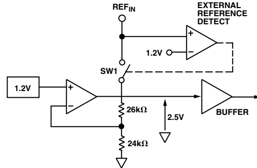
Figure 9. On-Chip Reference
