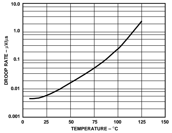
Droop Rate vs. Temperature, V_{IN} = 0\text{ V}
