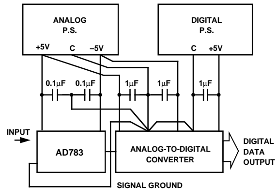
Figure 3. Basic Grounding and Decoupling Diagram
