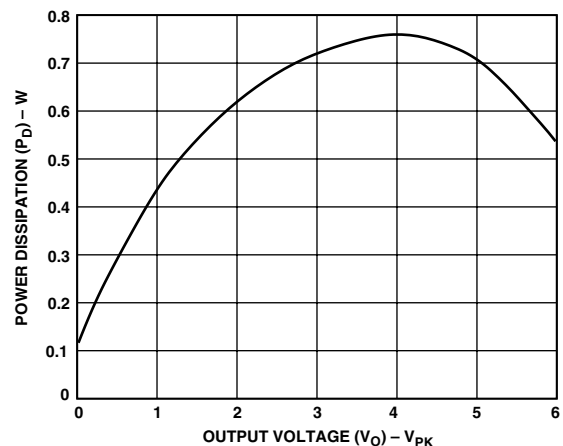
Figure 9. Power Dissipation ( P_D ) vs. Output Voltage ( V_O ), R_L = 50 \Omega
