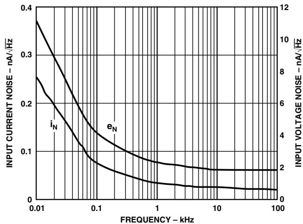
TPC 25. Noise vs. Frequency
