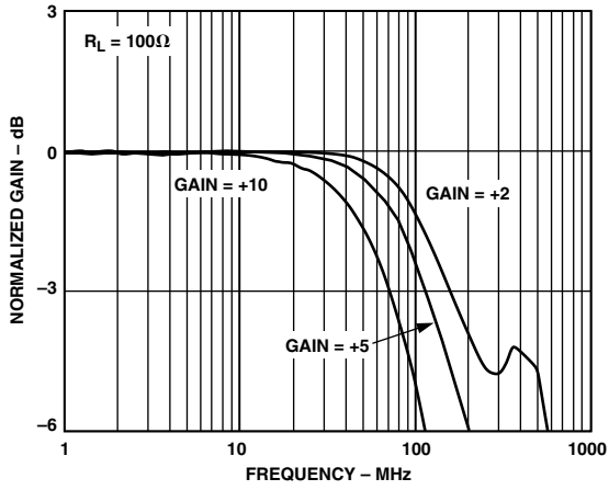
TPC 17. Frequency Response; V_S = \pm 6\text{ V}
