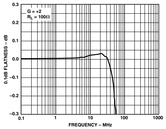
TPC 21. Gain Flatness; V_S = \pm 2.5\text{ V}
