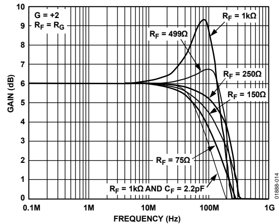
Figure 14. Small Signal Frequency Response vs. Frequency and R_F , Noninverting, V_{OUT} = 50 mV p-p (See Figure 48)
