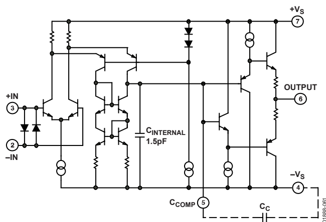
Figure 61. Simplified Schematic
