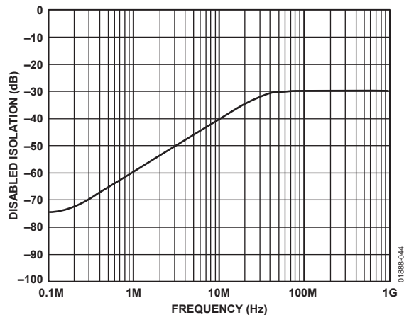
Figure 44. Input-to-Output Isolation, Chip Disabled (See Figure 54)
