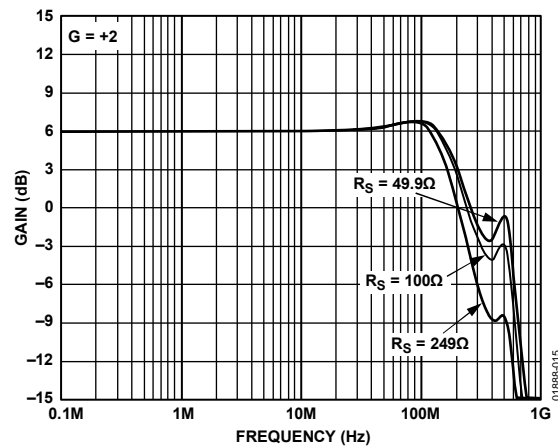
Figure 15. Small Signal Frequency Response vs. Frequency and R_S , Noninverting, V_{OUT} = 50 mV p-p (See Figure 48)
