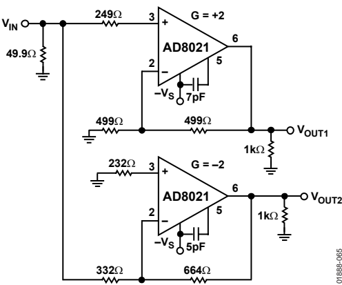
Figure 65. Differential Amplifier
