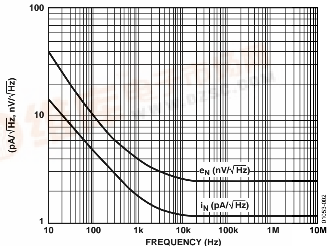
Figure 2. Current and Voltage Noise vs. Frequency
