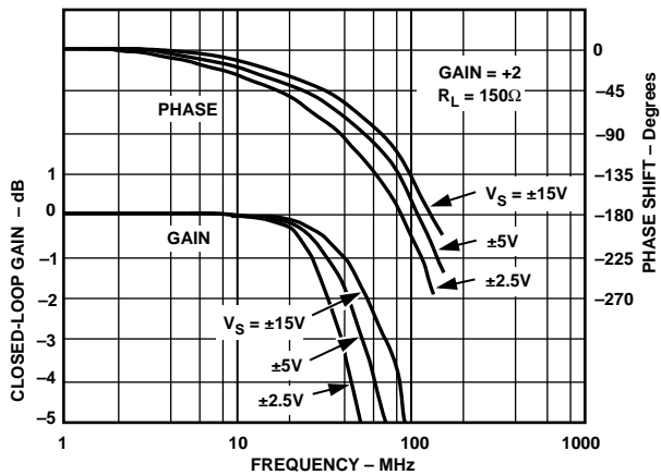
Figure 48. Closed-Loop Gain and Phase vs. Frequency, G = +2 , R_L = 150 , R_F = 715 \Omega
