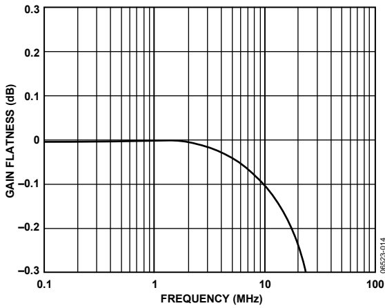
Figure 13. Small-Signal Gain Flatness, V_S = \pm 5\text{ V} , R_L = 150\ \Omega , V_{OUT} = 200\text{ mV p-p}
