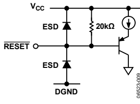
Figure 9. Reset Input
