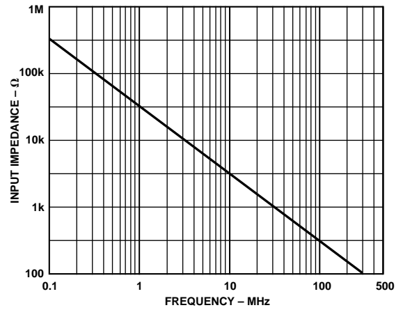
Figure 21. AD8115 Input Impedance vs. Frequency
