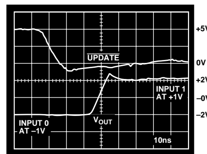
Figure 35. AD8115 Switching Time
