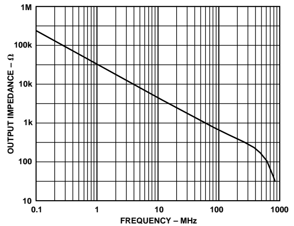
Figure 23. AD8115 Output Impedance, Disabled vs. Frequency
