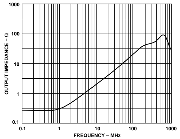
Figure 22. AD8115 Output Impedance Enabled vs. Frequency
