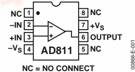
Figure 1. 8-Lead Plastic (N-8), Cerdip (Q-8), SOIC (R-8)
