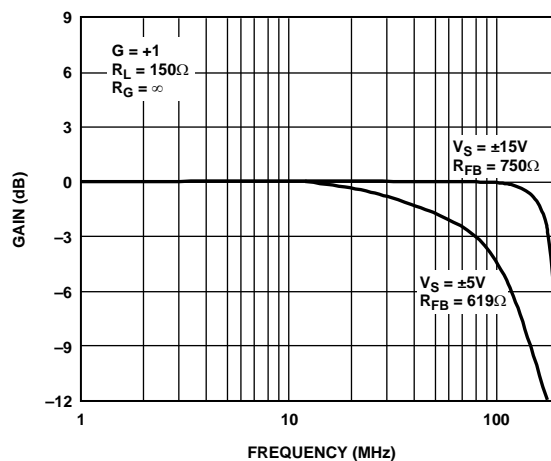
Figure 29. Closed-Loop Gain vs. Frequency, Gain = +1
