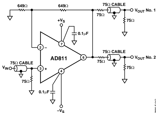
Figure 42. A Video Line Driver Operating at a Gain of +2
