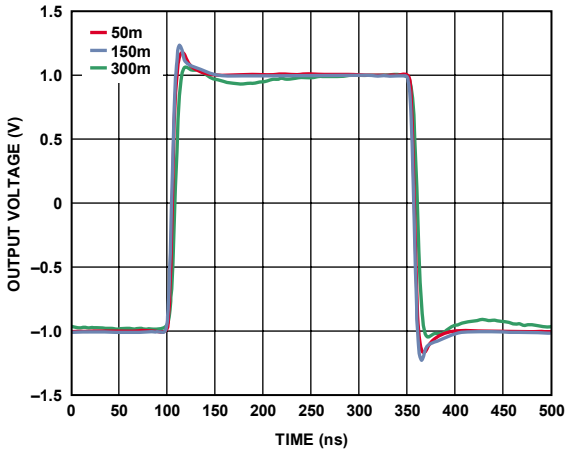
Figure 11. Pulse Response for Various Cable Lengths (2 MHz)
