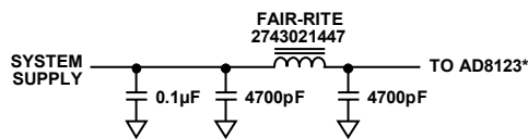
Figure 30. Power Supply Filter
