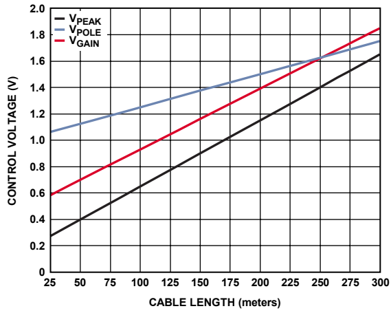
Figure 17. Recommended Settings for UTP Cable
