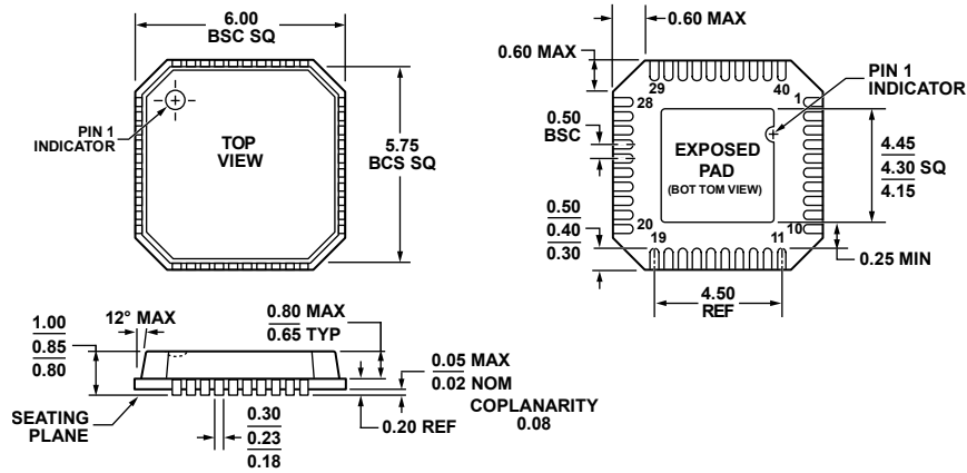
Figure 34. 40-Lead Lead Frame Chip Scale Package [LFCSP_VQ] 6 mm × 6 mm, Very Thin Quad (CP-40-4)
