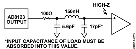
Figure 27. 140 MHz Low-Pass Filter on AD8123 Output Feeding High-Z Load
