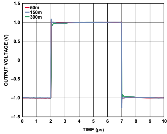
Figure 14. Pulse Response for Various Cable Lengths (100 kHz)
