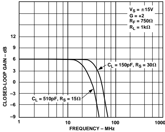
Figure 43. Response to Large Load Capacitor, V_S = \pm 15\text{ V}
