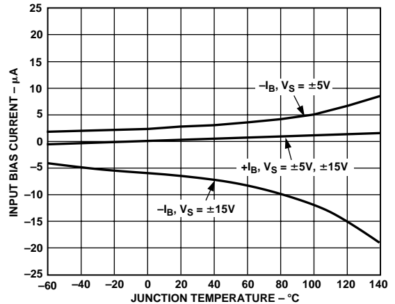
Figure 9. Input Bias Current vs. Junction Temperature
