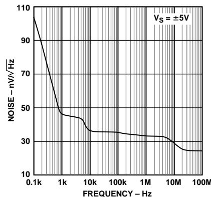
Figure 33. Voltage Noise vs. Frequency
