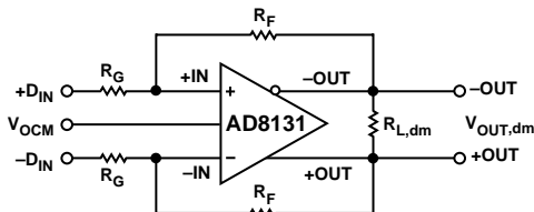
Figure 37. Circuit Definitions
