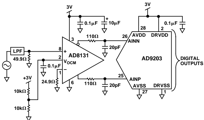
Figure 39. Test Circuit for AD8131 Driving an AD9203, 10 Bit, 40 Msp/s A-to-D Converter
