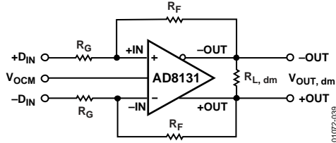
Figure 39. Circuit Definitions
