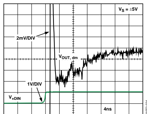
Figure 25. 0.1% Settling Time
