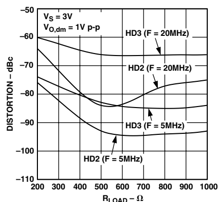
TPC 25. Harmonic Distortion vs. R_{LOAD} , G = 1
