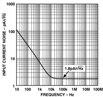
TPC 56. Input Current Noise vs. Frequency
