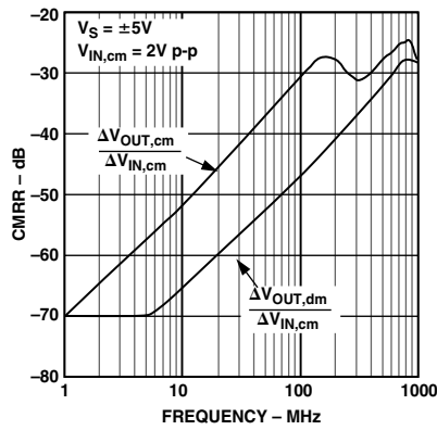
TPC 51. CMRR vs. Frequency
