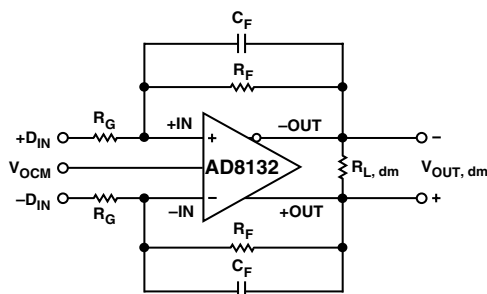
Figure 3. Circuit Definitions
