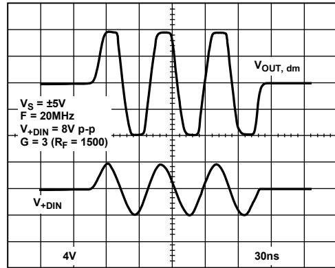
Figure 26. Output Overdrive
