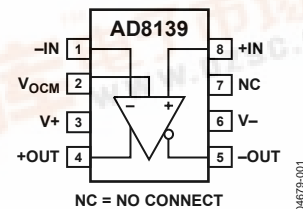
Figure 1. 8-Lead SOIC
