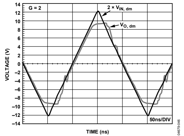
Figure 46. Overdrive Recovery
