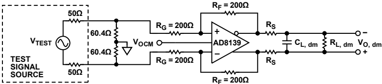
Figure 58. Capacitive Load Test Circuit, G = +1
