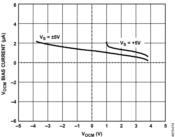
Figure 56. V OCM Bias Current vs. V OCM Input Voltage
