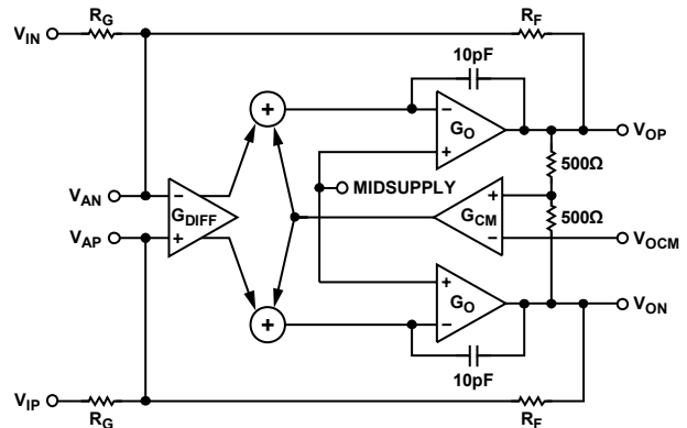
Figure 60. Block Diagram
