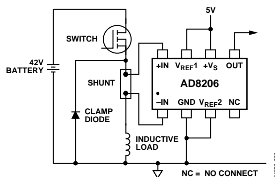
Figure 23. High-Side Switch
