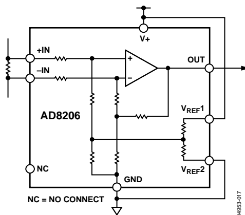
Figure 20. Split Supply
