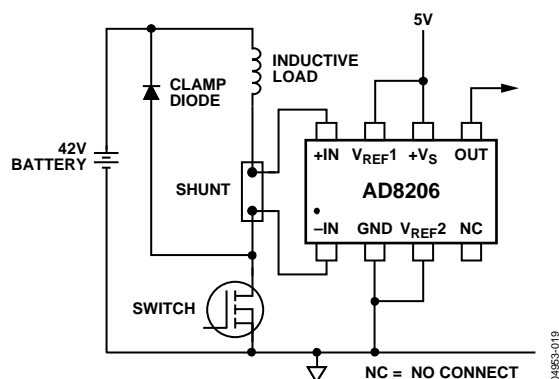
Figure 22. Low-Side Switch
