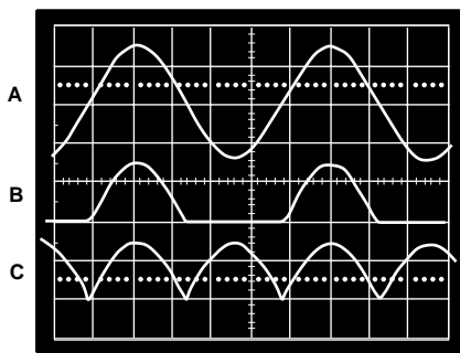
Figure 44. Single Supply Half- and Full-Wave Rectifier
