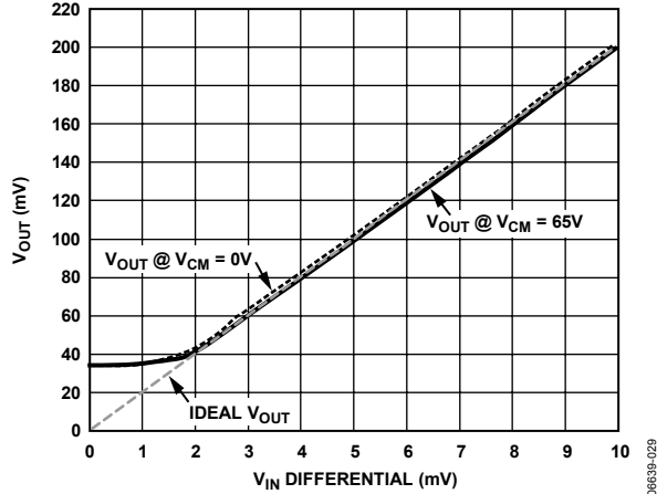
Figure 26. Gain Linearity Due to Differential and Common-Mode Voltage
