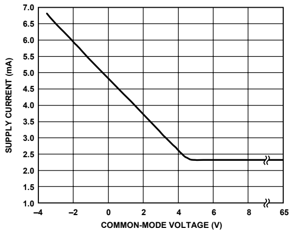
Figure 11. Supply Current vs. Common-Mode Voltage
