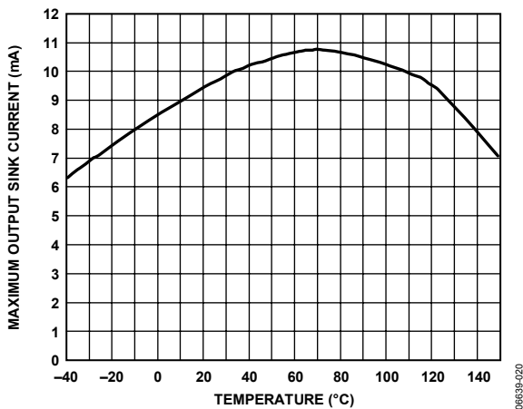
Figure 18. Output Sink Current vs. Temperature (Per Channel)
