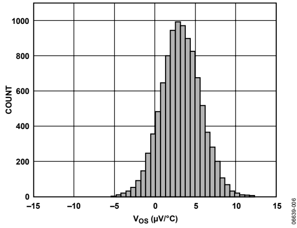
Figure 22. Offset Drift Distribution (µV/°C) (Temperature Range = -40°C to +125°C)
