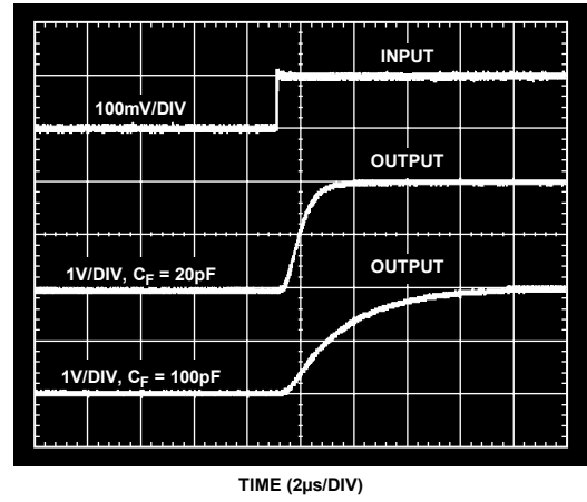
Figure 13. Rise Time
