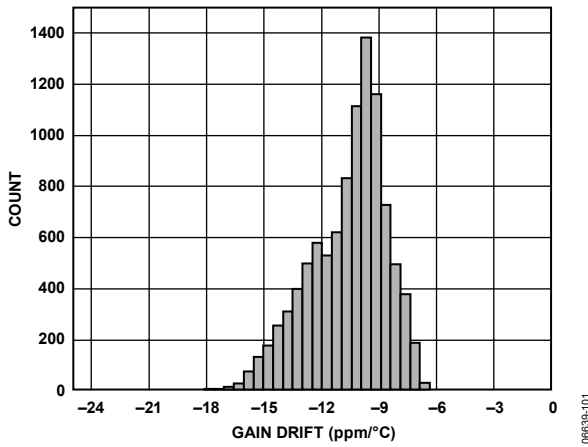
Figure 23. Gain Drift Distribution (ppm/°C) (Temperature Range = -40°C to +125°C)
