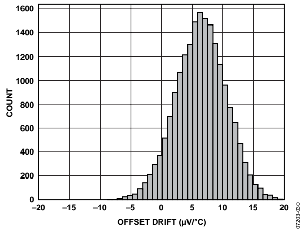
Figure 25. Offset Drift
