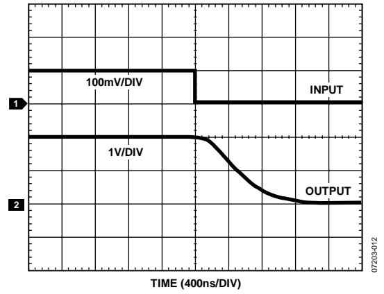
Figure 13. Fall Time
