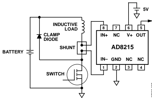
Figure 28. Low-Side Switch
