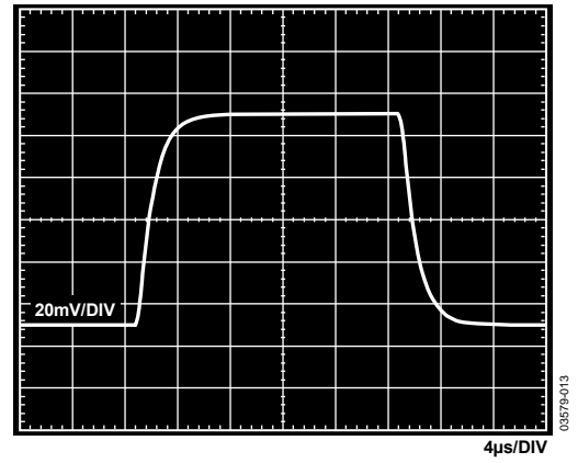
Figure 51. Small Signal Pulse Response, G = 100 , R_L = 2 \text{ k}\Omega , C_L = 100 \text{ pF} , V_S = +5 \text{ V} , V_{REF} = 2.5 \text{ V}
