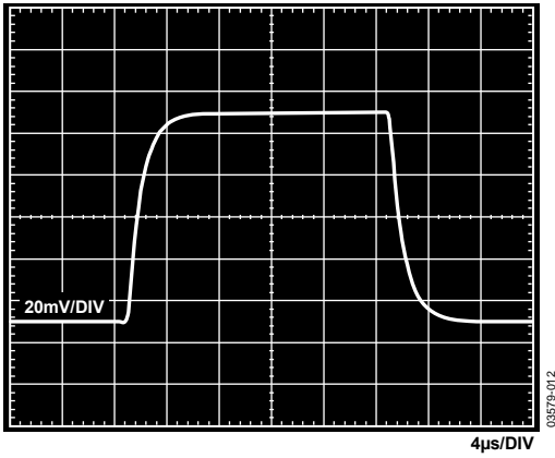
Figure 47 Small Signal Pulse Response, G = 100 , R_L = 2 \text{ k}\Omega , C_L = 100 \text{ pF} , V_S = \pm 15 \text{ V} , V_{REF} = 0 \text{ V}
