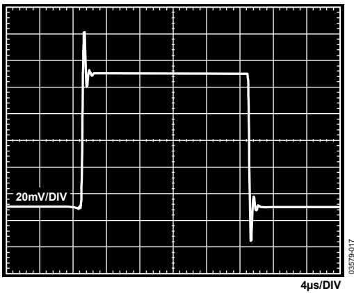
Figure 49. Small Signal Pulse Response, G = 1 , R_L = 2 \text{ k}\Omega , C_L = 100 \text{ pF} , V_S = +5 \text{ V} , V_{REF} = 2.5 \text{ V}
