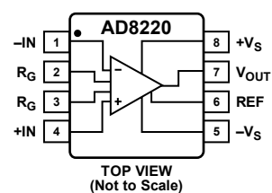
Figure 56. Pin Configuration
