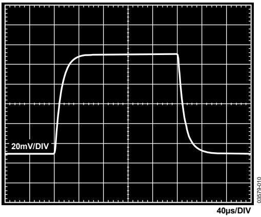
Figure 48. Small Signal Pulse Response, G = 1000 , R_L = 2 \text{ k}\Omega , C_L = 100 \text{ pF} , V_S = \pm 15 \text{ V} , V_{REF} = 0 \text{ V}
