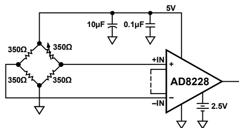
Figure 49. Precision Strain Gage
