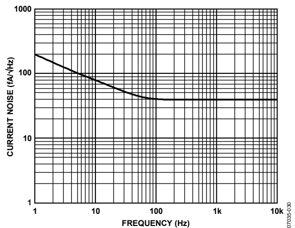
Figure 32. Current Noise Spectral Density vs. Frequency
