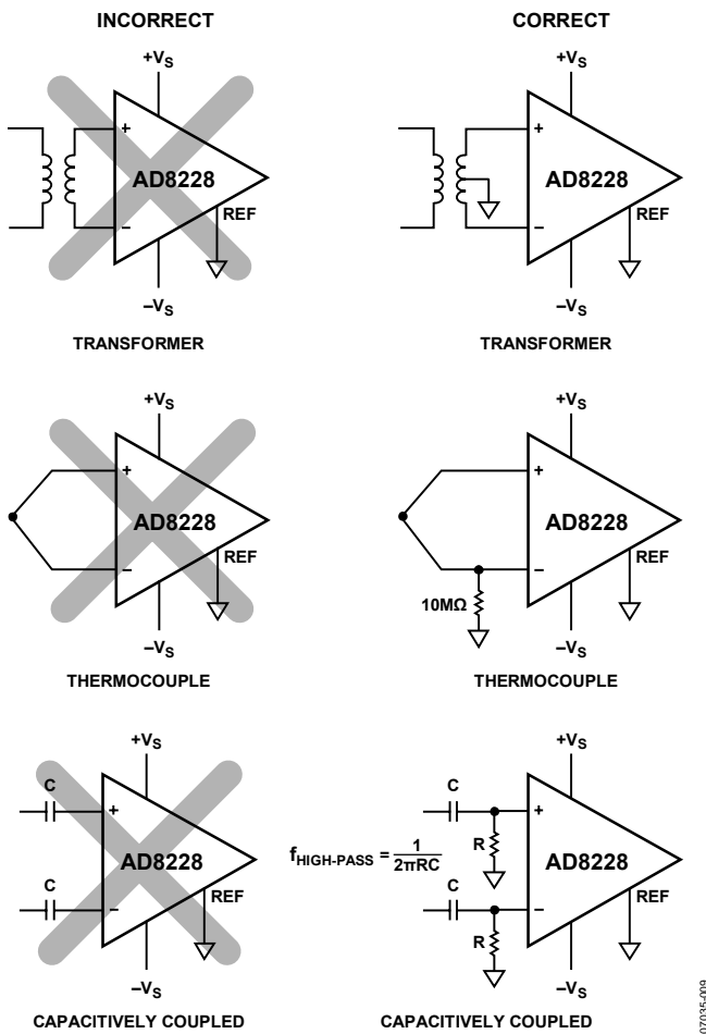
Figure 46. Creating an I_{BIAS} Path
