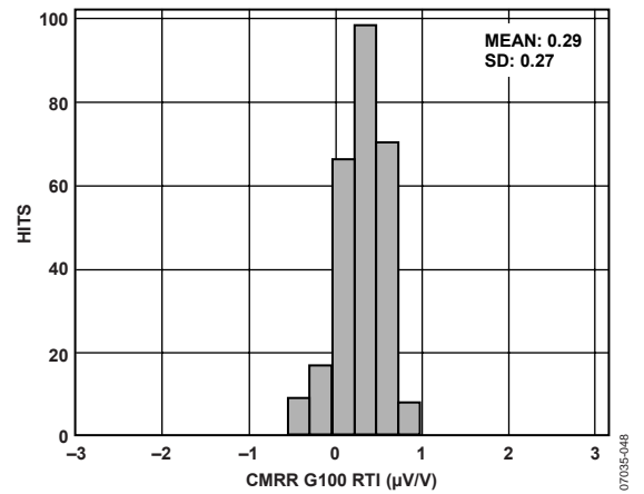
Figure 7. Typical Distribution for CMR (G = 100)
