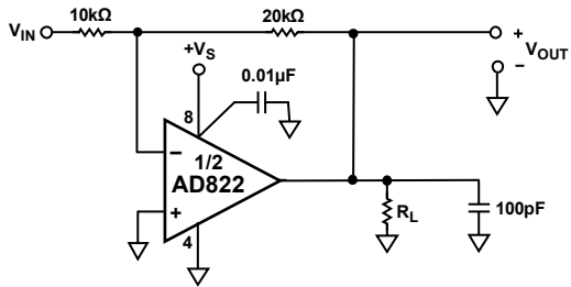
Figure 36. Gain-of-T2 Inverter
