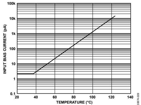
Figure 9. Input Bias Current vs. Temperature; V_S = 5\text{ V}, V_{CM} = 0
