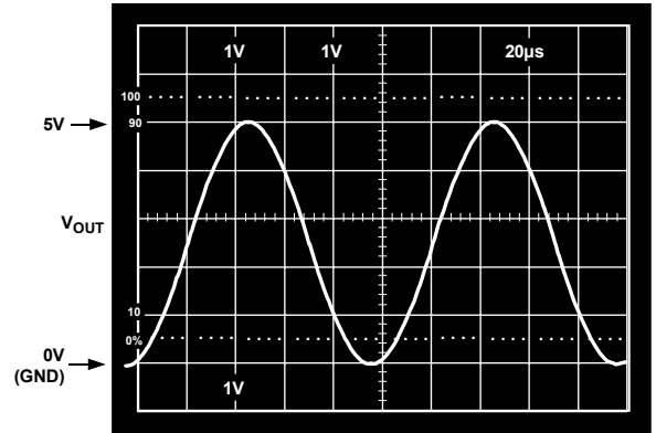
Figure 3. Gain-of-2 Amplifier; V_S = 5, 0 , V_{IN} = 2.5 \text{ V} Sine Centered at 1.25 V, R_L = 100 \Omega
